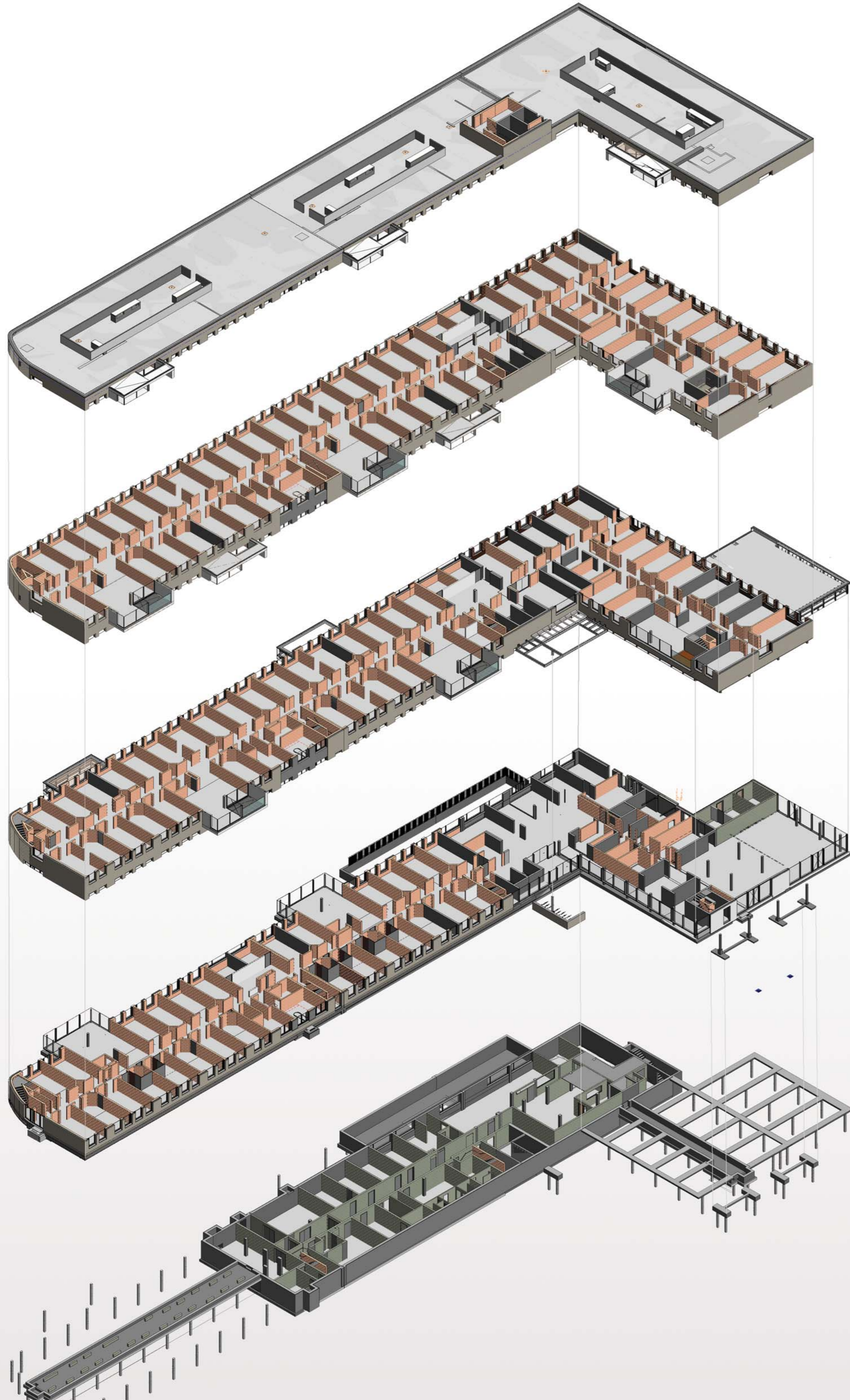
exploded view
